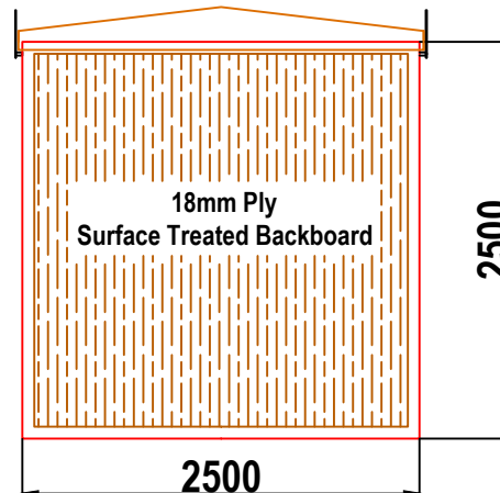
W6A WALK-IN GRP ENCLOSURE REAR WALL ELEVATION WALL 4
