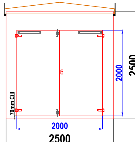
W6A WALK-IN GRP ENCLOSURE FRONT WALL ELEVATION WALL 1
