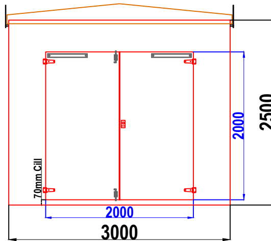
W7 WALK-IN GRP ENCLOSURE FRONT WALL ELEVATION WALL 1
