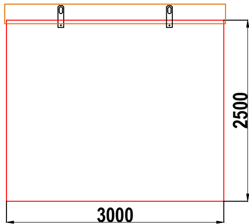
W7 WALK-IN GRP ENCLOSURE LEFT HAND SIDE WALL ELEVATION WALL 2
