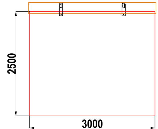
W7 WALK-IN GRP ENCLOSURE RIGHT HAND SIDE WALL ELEVATION WALL 3
