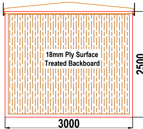
W7 WALK-IN GRP ENCLOSURE REAR WALL ELEVATION WALL 4
