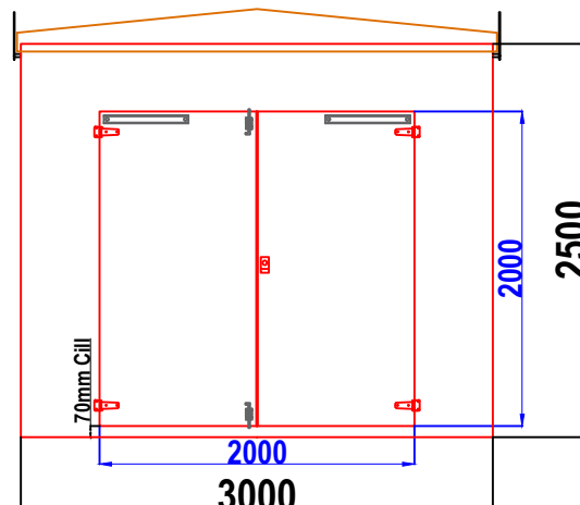
W7A WALK-IN GRP ENCLOSURE FRONT WALL ELEVATION WALL 1
