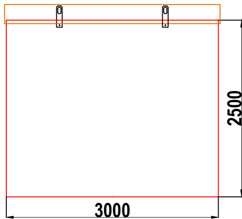
W7A WALK-IN GRP ENCLOSURE LEFT HAND SIDE WALL ELEVATION WALL 2
