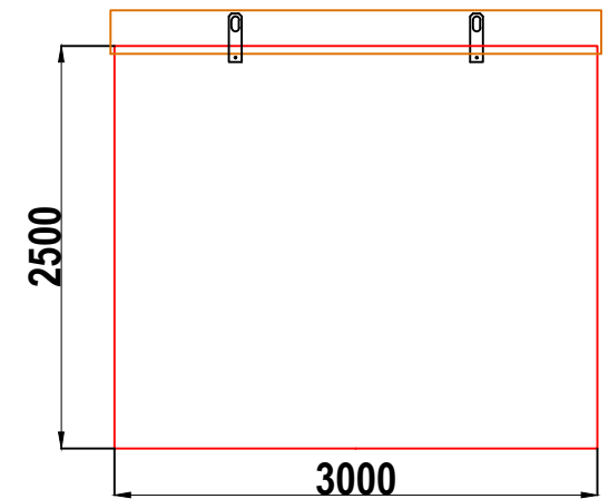
W7A WALK-IN GRP ENCLOSURE RIGHT HAND SIDE WALL ELEVATION WALL 3
