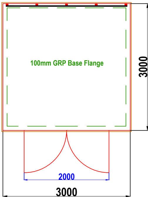
W7A WALK-IN GRP ENCLOSURE PLAN VIEW
