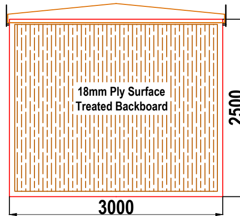
W7A WALK-IN GRP ENCLOSURE REAR WALL ELEVATION WALL 4
