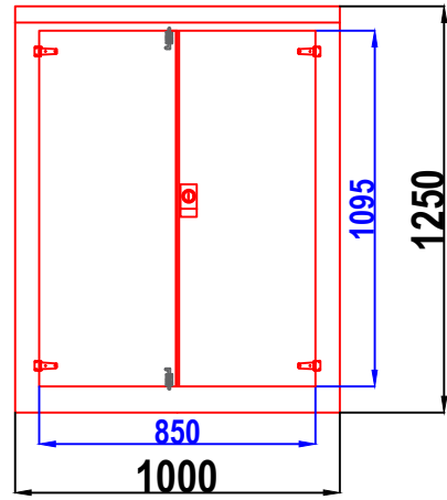
D1 GRP CABINET FRONT WALL ELEVATION WALL 1
