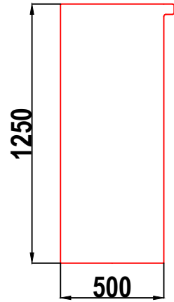
D1 GRP CABINET LEFT HAND SIDE WALL ELEVATION WALL 2
