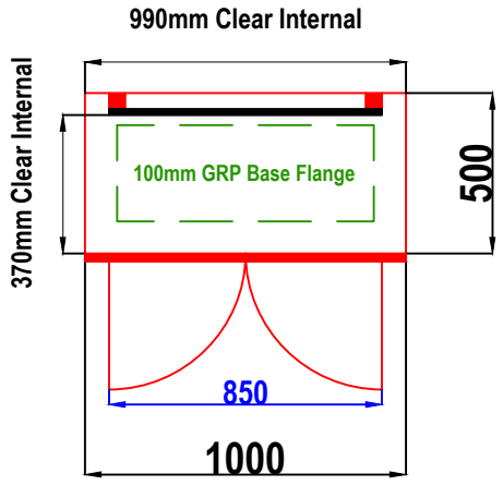
D1 GRP CABINET PLAN VIEW
