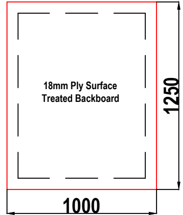
D1 GRP CABINET REAR WALL ELEVATION WALL 4
