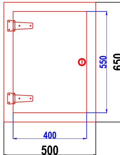
S1 GRP CABINET FRONT WALL ELEVATION WALL 1
