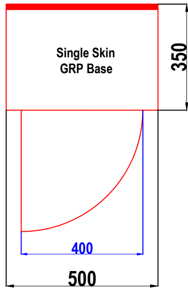
S1 GRP CABINET PLAN VIEW
