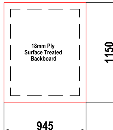
S3 GRP CABINET REAR WALL ELEVATION WALL 4
