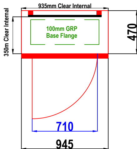
S3 GRP CABINET PLAN VIEW
