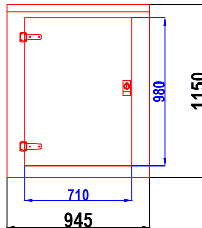
S3 GRP CABINET FRONT WALL ELEVATION WALL 1
