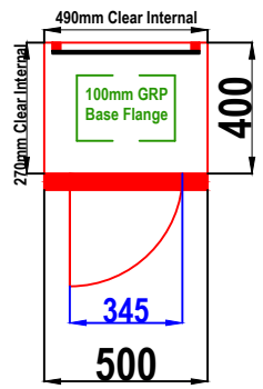
S4 GRP CABINET PLAN VIEW
