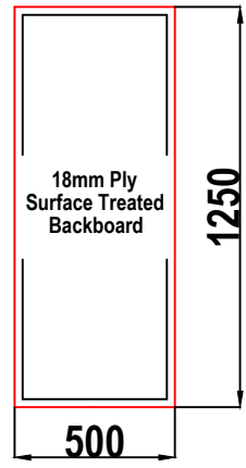
S4 GRP CABINET REAR WALL ELEVATION WALL 4
