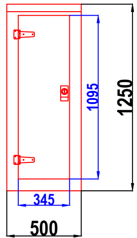
S4 GRP CABINET FRONT WALL ELEVATION WALL 1
