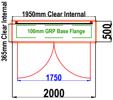
W1 GRP WALK-IN CABINET PLAN VIEW
