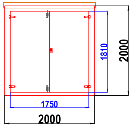
W1 GRP WALK-IN CABINET FRONT WALL ELEVATION WALL 1
