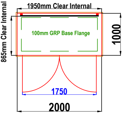
W2 GRP WALK-IN CABINET PLAN VIEW
