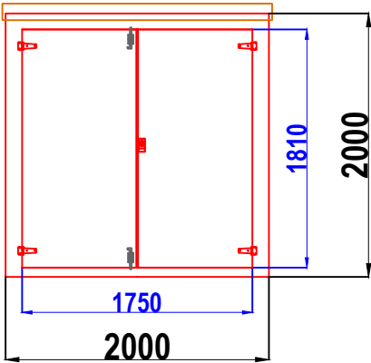
W2 GRP WALK-IN CABINET FRONT WALL ELEVATION WALL 1
