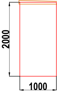
W2 GRP WALK-IN CABINET RIGHT HAND SIDE WALL ELEVATION WALL 3
