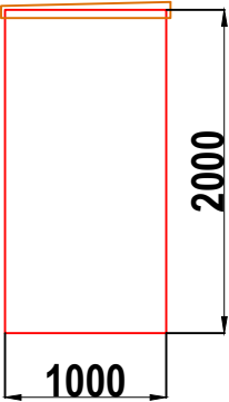
W2 GRP WALK-IN CABINET LEFT HAND SIDE WALL ELEVATION WALL 2
