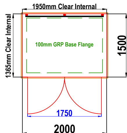
W3 GRP WALK-IN CABINET PLAN VIEW
