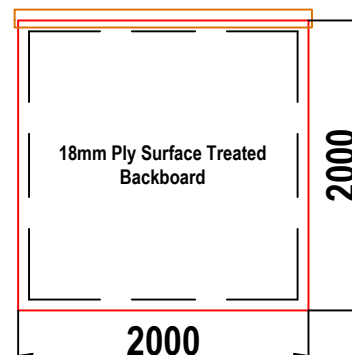
W3 GRP WALK-IN CABINET REAR WALL ELEVATION WALL 4
