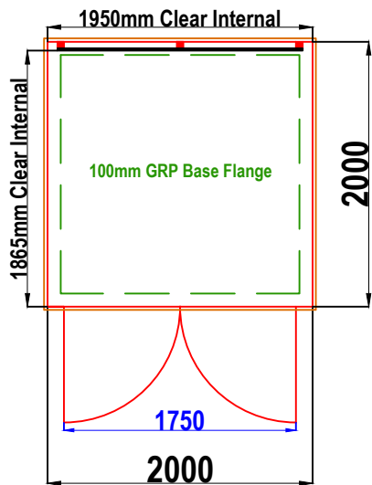
W4 GRP WALK-IN CABINET PLAN VIEW
