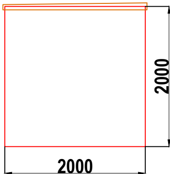
W4 GRP WALK-IN CABINET LEFT HAND SIDE WALL ELEVATION WALL 2
