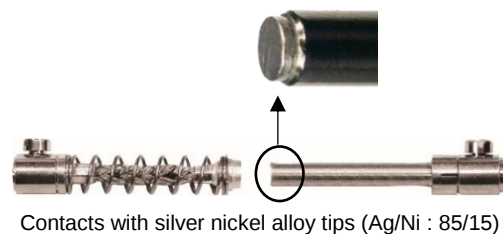
Contacts with silver nickel alloy tips (Ag/Ni : 85/15)
