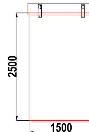
W10 WALK-IN GRP ENCLOSURE RIGHT HAND SIDE WALL ELEVATION WALL 3
