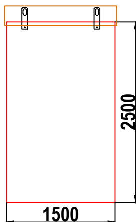
W10 WALK-IN GRP ENCLOSURE LEFT HAND SIDE WALL ELEVATION WALL 2
