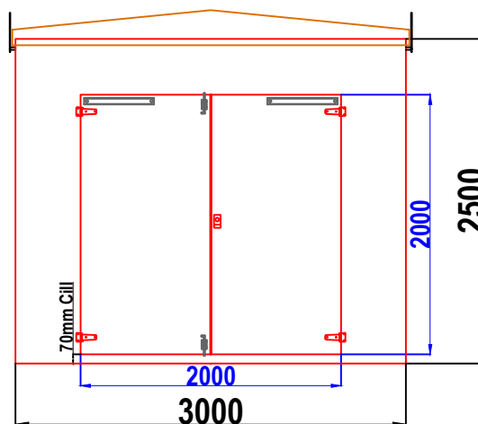
W10 WALK-IN GRP ENCLOSURE FRONT WALL ELEVATION WALL 1
