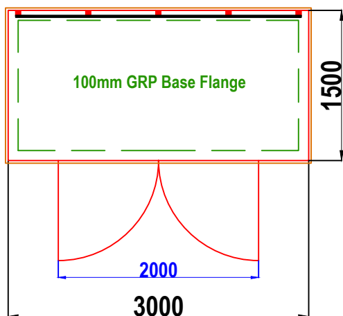
W10 WALK-IN GRP ENCLOSURE PLAN VIEW
