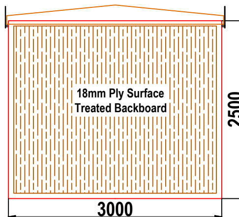
W10 WALK-IN GRP ENCLOSURE REAR WALL ELEVATION WALL 4
