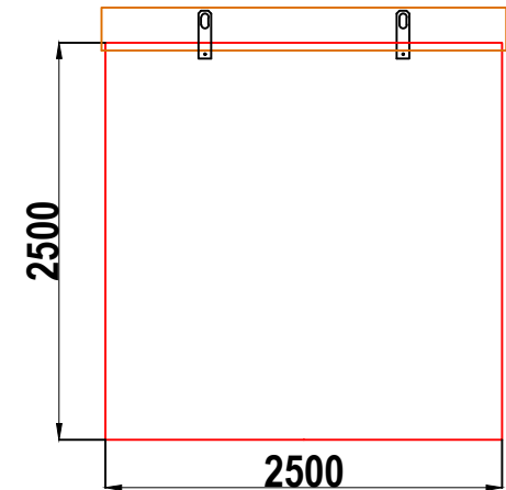
W12 WALK-IN GRP ENCLOSURE RIGHT HAND SIDE WALL ELEVATION WALL 3
