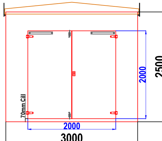
W12 WALK-IN GRP ENCLOSURE FRONT WALL ELEVATION WALL 1
