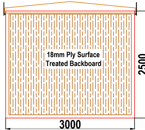
W12 WALK-IN GRP ENCLOSURE REAR WALL ELEVATION WALL 4
