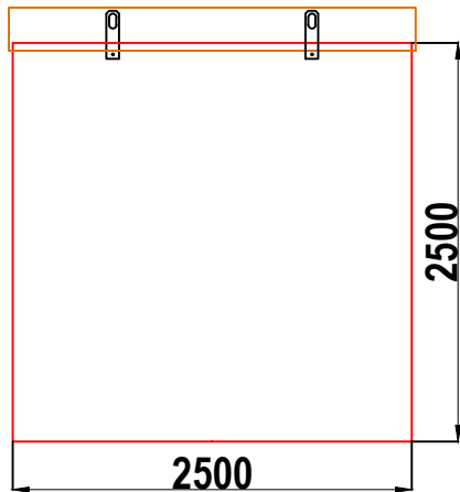
W12A WALK-IN GRP ENCLOSURE LEFT HAND SIDE WALL ELEVATION WALL 2
