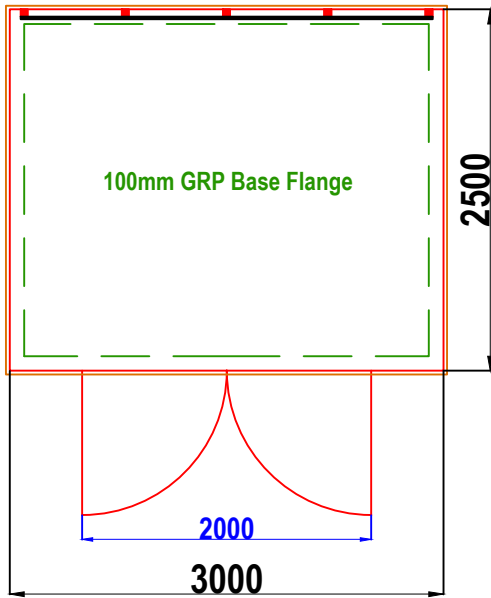
W12A WALK-IN GRP ENCLOSURE PLAN VIEW
