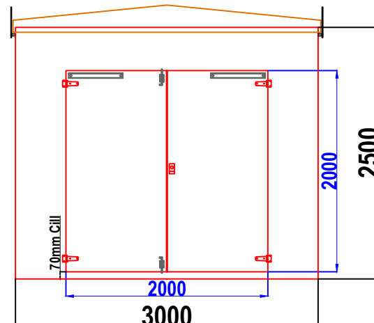
W12A WALK-IN GRP ENCLOSURE FRONT WALL ELEVATION WALL 1
