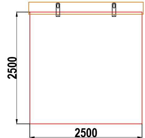
W12A WALK-IN GRP ENCLOSURE RIGHT HAND SIDE WALL ELEVATION WALL 3
