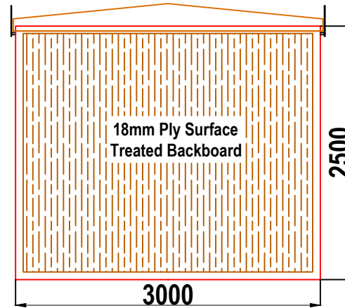
W12A WALK-IN GRP ENCLOSURE REAR WALL ELEVATION WALL 4
