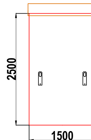
W8 WALK-IN GRP ENCLOSURE RIGHT HAND SIDE WALL ELEVATION WALL 3
