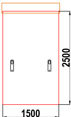
W8 WALK-IN GRP ENCLOSURE LEFT HAND SIDE WALL ELEVATION WALL 2
