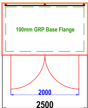
W8 WALK-IN GRP ENCLOSURE PLAN VIEW
