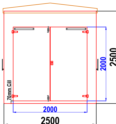
W8 WALK-IN GRP ENCLOSURE FRONT WALL ELEVATION WALL 1
