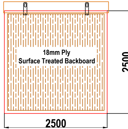
W9A WALK-IN GRP ENCLOSURE REAR WALL ELEVATION WALL 4
