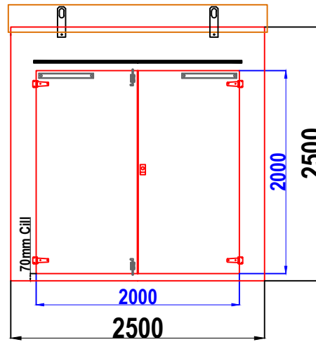
W9A WALK-IN GRP ENCLOSURE FRONT WALL ELEVATION WALL 1
