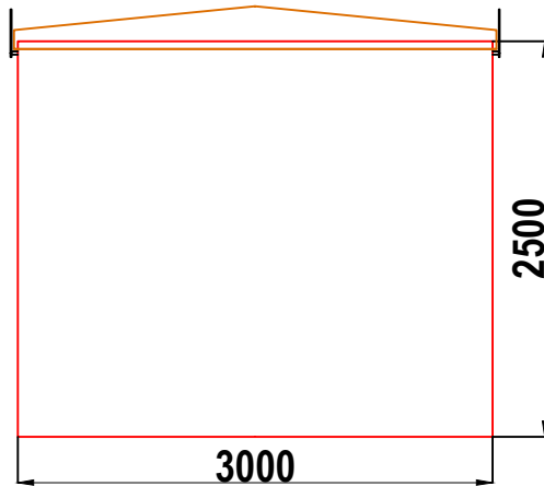
W9A WALK-IN GRP ENCLOSURE LEFT HAND SIDE WALL ELEVATION WALL 2
