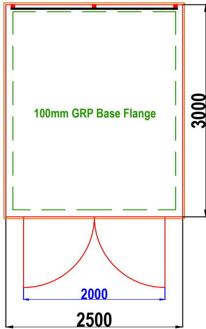
W9A WALK-IN GRP ENCLOSURE PLAN VIEW
