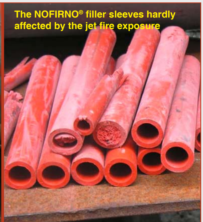
The NOFIRNO ® filler sleeves hardly affected by the jet fire exposure
