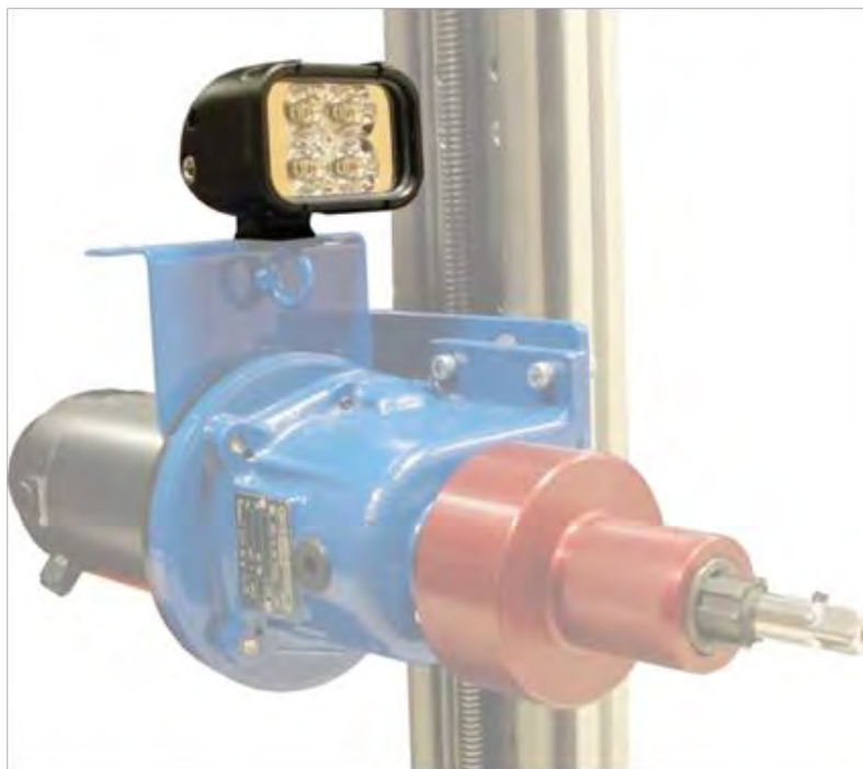
Figure E-1: LED Light installed on RRS-1
