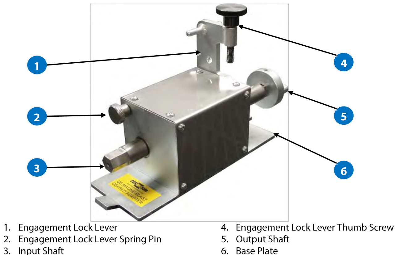
Figure I-2: Magne-blast Geared Adapter
