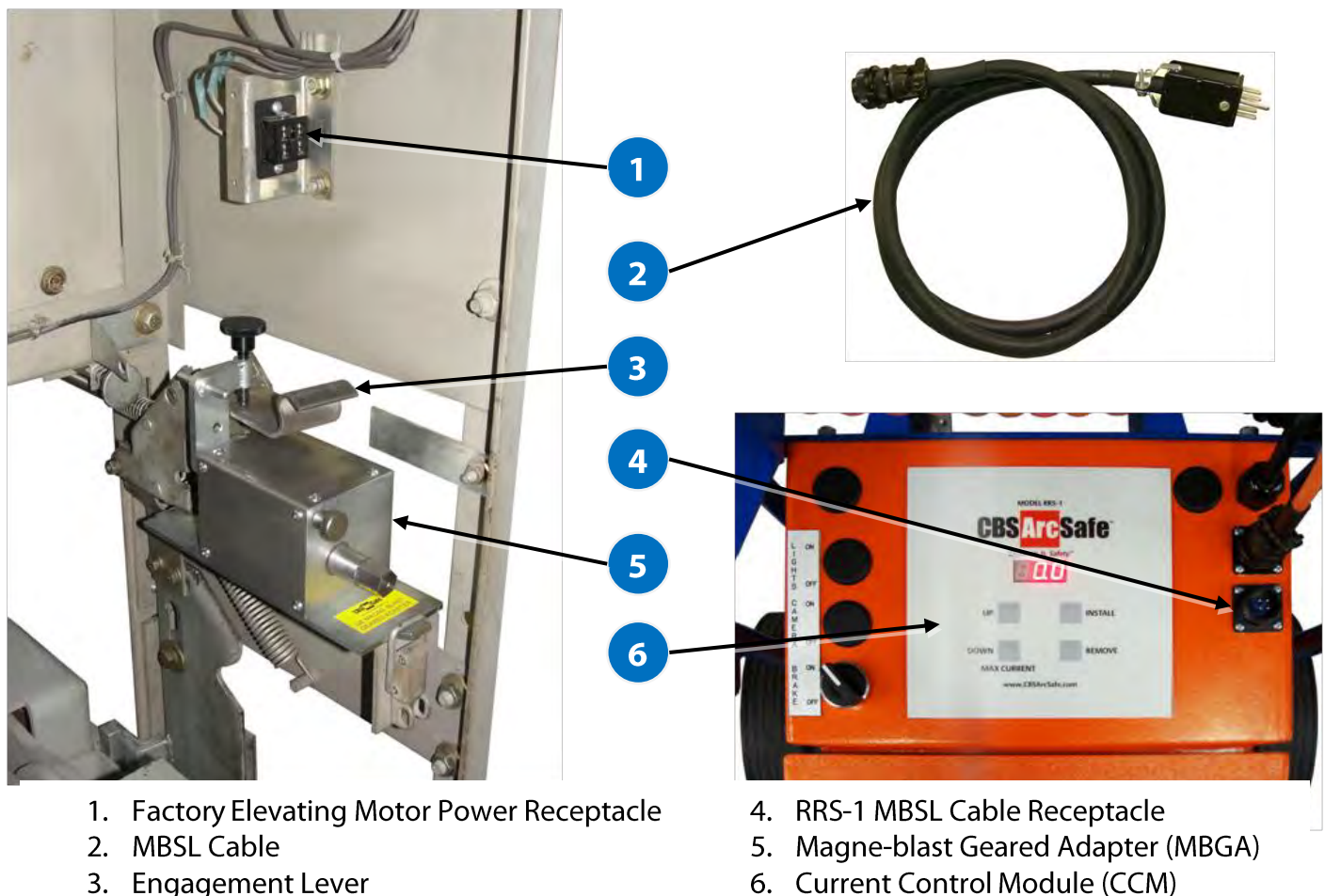
Figure I-1: MBSL Components
