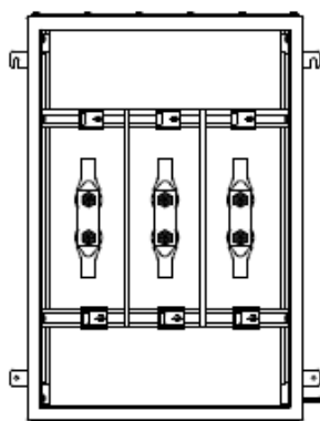
HVJB X3 (1-1) Cables entering from top and bottom
