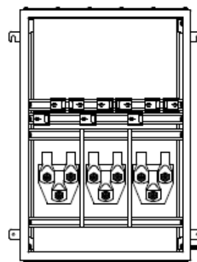
HVJB X3 (3-0) Cables entering from top only
