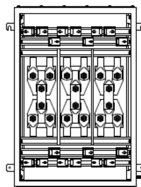
HVJB X3 (3-3) Cables entering from top and bottom
