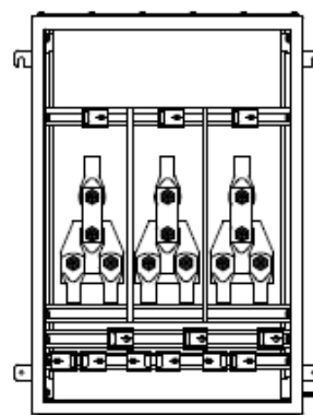
HVJB X3 (1-3) Cables entering from top and bottom
